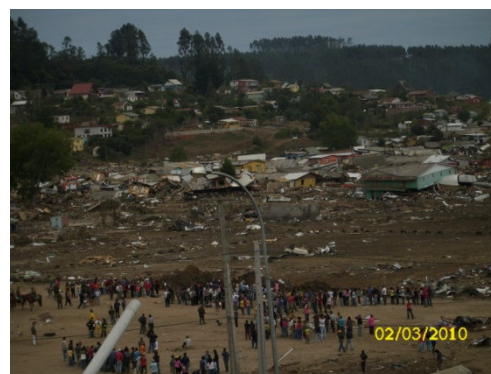
Dichato after 2010 Chilean Tsunami
